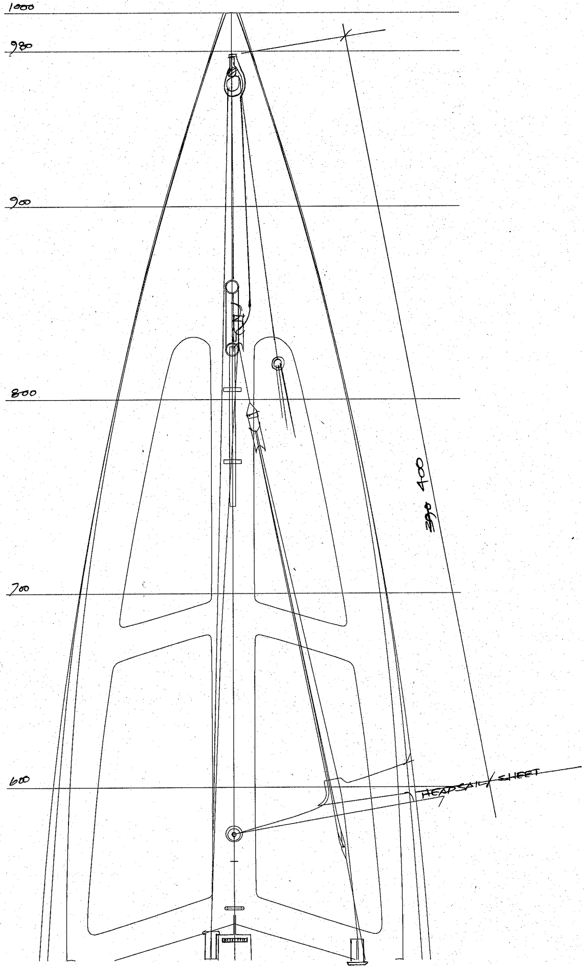
Plan View
